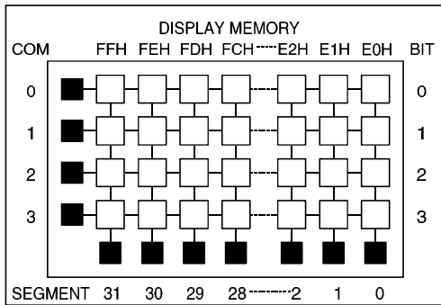
HT44300 LCD Display Memory
