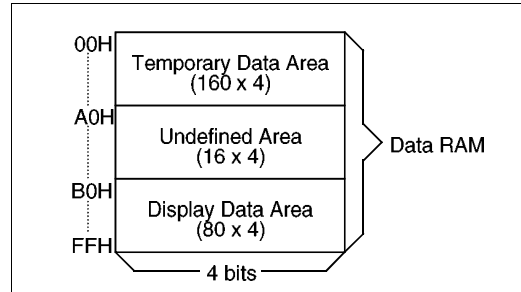
HT443A0 Data Memory
