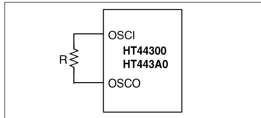
RC Oscillator
