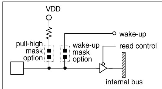
Input Ports PP, PS, PM
