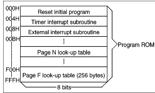
Program Memory
