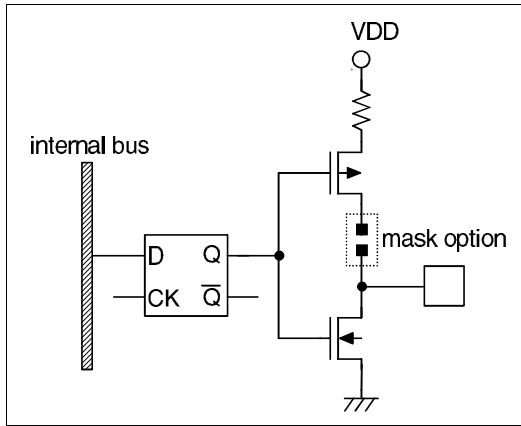
Output Port PA
