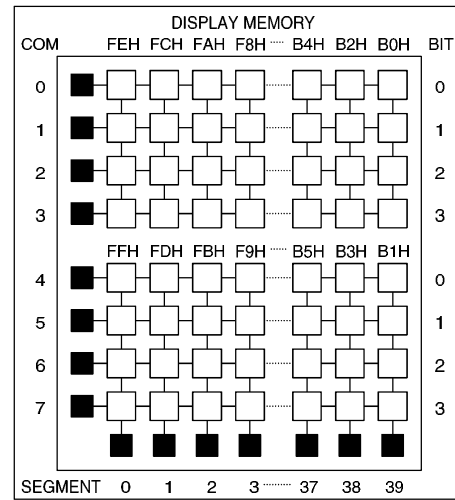
HT443A0 LCD Display Memory
