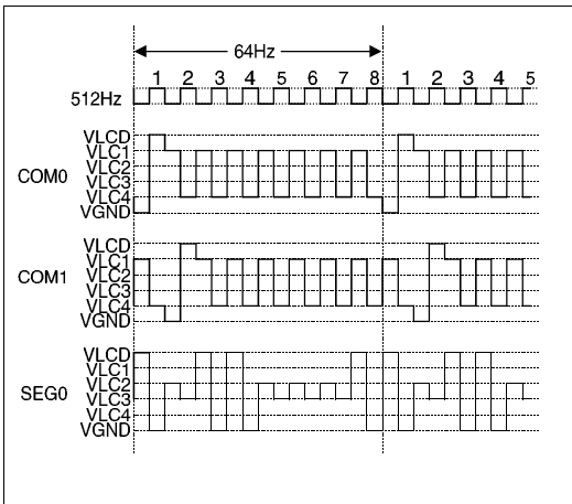
HT443A0 LCD Driver Output
