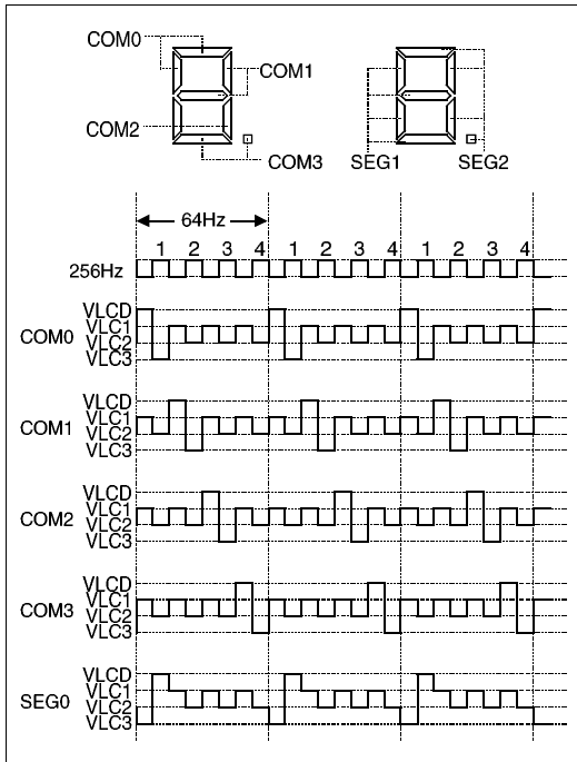
HT44300 LCD Driver Output
